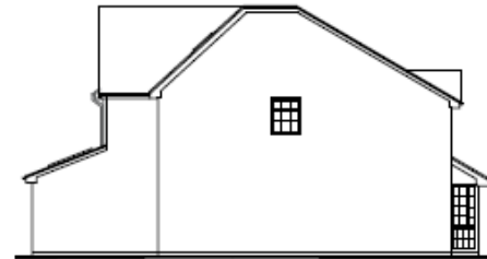
Proposed Side Elevation Scale 1:100
